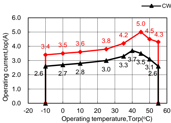
Fig.1 The relation of operating temperature vs maximum operating current
